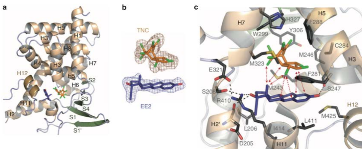
Figure 8: Synergy between EDs - Example of a supra-molecular ligand composed of trans-nonachlor and 17-ethinyl-oestradiol. a) Pregnane-X receptor (PXR) in which trans-nonachlor (TNC) and 17-EE (EE2) are bound. b) TNC and EE2 molecules. c) Visualization of the interactions between the molecules TNC and EE2, creating a supra-molecular ligand in the ligand-binding pocket of PXR [82].
